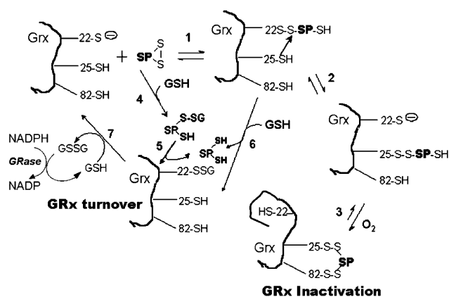
FIGURE 11: Mechanistic models of sporidesmin as a substrate and inactivator of GRx1. This scheme shows two alternative explanations for sporidesmin as a substrate of GRx1: (a) steps 4, 5, and 7 depict an initial nonenzymatic formation of glutathionyl mixed disulfide of sporidesmin, sporidesmin-SSG, which is then reduced by GSH in a GRx1 catalyzed reaction to form reduced sporidesmin. This postulated mechanism is consistent with the two-substrate kinetics (Figure 1) and previous characterization of the substrate specificity of GRx1 and the mode of substrate activity of non-GSH-containing disulfides as reported previously (1, 2, 4, 5). (b) Steps 1, 6, and 7 depict the direct reaction of sporidesmin with GRx1 to form GRx1 sporidesmin mixed disulfide (GRx1-S-S-sporidesmin). GSH then displaces sporidesmin from this adduct to form GRx1-SSG, which can enter the normal catalytic cycle of GRx1. (c) When GSH is scarce or absent, the GRx1-S-S-sporidesmin complex goes on to an irreversibly inactivated form according to steps 1, 2, and 3 involving molecular oxygen.
