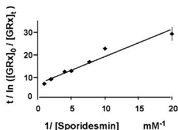
FIGURE 3: Modified Kitz–Wilson plot for GRx1 inactivation by sporidesmin. GRx1 (0.9 \mu M) was incubated with different concentrations of sporidesmin (0.05–1 mM) for 5 min at 30 °C, 0.1 M K phosphate, pH 7.5, and residual activities were determined relative to ethanol treated control as described in Figure 2. K_i and k_{\text{inact}} were determined according to the relationship \ln(E_0/E_t)/t = k_{\text{inact}}[I]/(K_i + [I]) , where E_0 and E_t refer to GRx1 concentrations at times 0 and t , [I] refers to sporidesmin concentration, K_i is the concentration of inactivator that gives half the maximal rate of inactivation, and k_{\text{inact}} is the net rate constant for inactivation. The K_i of sporidesmin for GRx1 is 0.15 mM, and the k_{\text{inact}} is 0.72 min −1 . Each point represents the mean value, plus and minus the standard error, for at least three determinations. Where error bars are not evident, they are within the size of the symbol.
