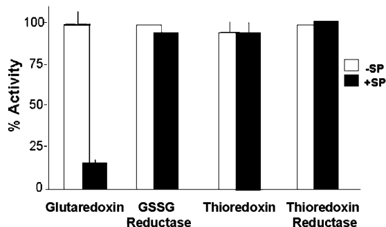
FIGURE 4: Selective inactivation of GRx1 by sporidesmin. Thiol-disulfide oxidoreductase enzymes were incubated with 1 mM sporidesmin at 30 °C, 0.1 M K phosphate (5% ethanol), pH 7.5 for 20 min. The remaining enzyme activity was expressed as percent of the control activity. Human GRx1 (1.8 \mu M) activity was determined by GSSG-reductase mediated NADPH oxidation coupled to GSSG formation. Yeast GSSG reductase (0.125 \mu M) activity was measured by the loss of NADPH absorbance at 340 nm. E. coli thioredoxin (0.2 mg mL −1 ) and thioredoxin reductase (0.1 mg mL −1 ) were assayed by NADPH oxidation coupled to thioredoxin oxidation using GSSG as the substrate. Mammalian thioredoxin was assayed by a turbidometric assay using insulin as the substrate. Each bar represents the mean value, plus and minus the standard error, for at least three determinations. Where errors are not shown, the value represents a single experiment carried out after optimization of conditions.
