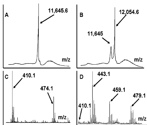
FIGURE 8: Mass spectrometry of GRx1, sporidesmin, and reaction products. MALDI spectra of GRx1 and the reaction product with sporidesmin show ions at m/z 11 645 corresponding to native GRx1 (A), and m/z 12 054 consistent with formation of a mixed disulfide between GRx1 and sporidesmin followed by elimination of two sulfur atoms (B). ESI spectra of sporidesmin (C) and the corresponding low mass regions in the product of reaction with GRx1 (D) contain ions consistent with the presence of sporidesmin (calculated m/z 474.0555), sporidesmin minus two sulfur atoms (calculated mass 410.1113), and in the reaction product ions corresponding to sporidesmin in which a sulfur has been replaced by hydrogen (calculated m/z 443.0912) and the product of monooxygenation of the remaining sulfur atom (calculated m/z 459.0862). The identity of the m/z 479 species is unknown. Low mass regions of the spectra were internally calibrated using the sporidesmin ion.
