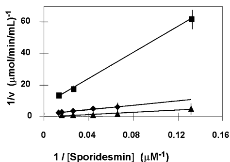
FIGURE 1: Two-substrate kinetics for GSH-dependent GRx1-catalyzed reduction of sporidesmin. Two-substrate kinetics for sporidesmin and glutathione with GRx1. Concentrations of GSH and sporidesmin were varied in the presence and absence of GRx1. The two-substrate kinetic analysis of sporidesmin (7.6–76 \mu\text{M} ) and GSH (0.4 mM, solid square; 2 mM, solid diamond; 5 mM, solid triangle) with GRx1 (0.035 \mu\text{M} ) shows an intersecting pattern of lines consistent with a sequential mechanism. Each point represents the mean value, plus and minus the standard error, for at least three determinations. Where error bars are not evident, they are within the size of the symbol.
