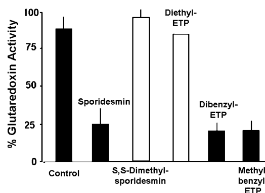
FIGURE 5: Reaction of ETP analogues with GRx1. Structural requirements for inactivation. GRx1 (2 \mu M) was treated with different ETP analogues at 1 mM final concentration. The synthetic ETPs were dissolved in dimethyl sulfoxide to a final concentration of 100 mM and diluted 1/100 into the GRx1-containing solution at 0.1 M K phosphate, pH 7.5, 30 °C. GRx1 was treated with 1% ethanol or dimethyl sulfoxide as controls for these experiments. After incubation for 20 min, the samples were assayed for GRx1 activity using cys-SSG as the substrate. Each bar represents the mean value, plus and minus the standard error, for at least three determinations. In the case of diethyl-ETP, no error is shown because this represents a single experiment after optimization of conditions, due to limited supply of this ETP derivative.
