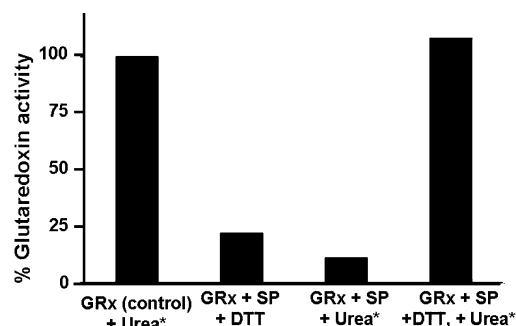
FIGURE 6: Requirements for reactivation of sporidesmin-inactivated GRx1. GRx1 (100 \mu M) was treated with either 1 mM sporidesmin or 5% ethanol at 30 °C, 0.1 M K phosphate, pH 7.5. Enzyme activity was measured after incubation for 15 min. The sporidesmin-treated sample was approximately 90% inactivated. The control was treated with 8 M urea plus 50 mM DTT. The inactivated GRx1 was divided into two aliquots and treated with either 8 M urea or 50 mM DTT and 8 M urea. The samples (including urea plus DTT treated control) were each loaded on a gel filtration column and separated from excess small molecules. The GRx1 protein was pooled and analyzed for activity and protein content. The results shown in the figure are for a single experiment, after conditions were optimized. The recovery of protein after size exclusion chromatography was 55–60% for all three samples. GRx1 inactivated with sporidesmin and exposed to urea alone or DTT alone showed no reactivation, while treatment with sporidesmin and then urea plus DTT gave 60% recovery of activity, i.e., full recovery of GRx activity when normalized to 55–60% protein recovery.
