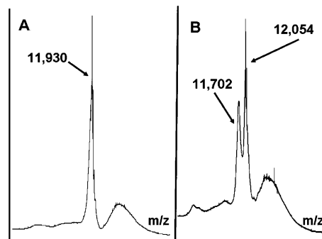
FIGURE 9: Alkylation of GRx1 cysteines with iodoacetamide (IAM). MALDI spectra of GRx1 reacted with iodoacetamide (A), and GRx1 first reacted with sporidesmin and then with iodoacetamide (B). IAM-treated GRx1 contained a major ion m/z 11 930 \pm 3 consistent with alkylation of all five cysteines. MALDI analysis of the products of reaction of GRx1 with sporidesmin, then treated with IAM, only showed major ions corresponding to the SP-GRx1 adduct ( m/z 12 054) and GRx1 modified by carboxamidomethylation of a single cysteine (calculated m/z 11 702).
