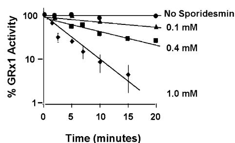
FIGURE 2: Inactivation of GRx1. Time- and concentration-dependent loss of GRx1 activity. GRx1 (2–10 \mu\text{M} ) was treated with different concentrations (0.1–1 mM) of sporidesmin in 0.1 M K phosphate, pH 7.5, 10% ethanol. At different times, aliquots were tested for GRx1 activity according to the spectrophotometric assay (GSSG-reductase mediated NADPH oxidation coupled to GSSG formation) using cys-SSG as the prototype substrate. In parallel, rates of NADPH oxidation for equivalent aliquots were determined in the absence of cys-SSG to account for the effect of residual sporidesmin transferred to the assay with the deactivated GRx1. These small non-cys-SSG-dependent rates were subtracted from the overall rates observed with cys-SSG to obtain the data for each point shown in Figure 2. Each point represents the mean value, plus and minus the standard error, for at least three determinations. Where error bars are not evident they are within the size of the symbol.
