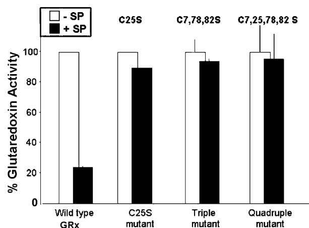
FIGURE 7: Study of sporidesmin reaction with cysteine-to-serine mutants of GRx1. Site-directed mutagenesis was utilized to produce the cys to ser mutant GRx1 enzymes, as described in Methods. Each enzyme (3–5 \mu M) was incubated with 1 mM sporidesmin for 20 min in 0.1 M K phosphate, pH 7.5, 10% ethanol at 30 °C. GRx1 activity was then measured using cys-SSG substrate. Each point represents the mean value, plus and minus the standard error, for at least three determinations. Where errors are not shown, the value represents a single experiment carried out after optimization of conditions.
