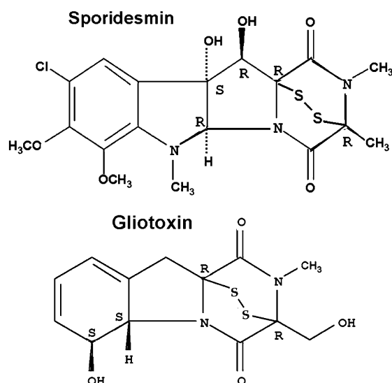
Chart 1: Structures of Sporidesmin and Gliotoxin a
