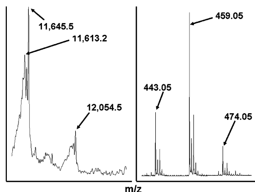
FIGURE 10: Reaction of GRx1 and adduct with DTT. GRx1 was pretreated with sporidesmin, followed by incubation in the presence of 35 mM DTT for 1 h at room temperature, and then subjected to mass spectral analysis. MALDI ions at m/z 11 613 \pm 2 and 443 were consistent with release of GRx1 and sporidesmin, respectively, each less a sulfur atom, as would be expected if two sulfurs had been eliminated from the adduct. Ions consistent with the presence of unreacted GRx1 (11 645) and SP-GRx1 adduct minus 64 Da (12 054), reflecting possible loss of two sulfur atoms, are also evident.
